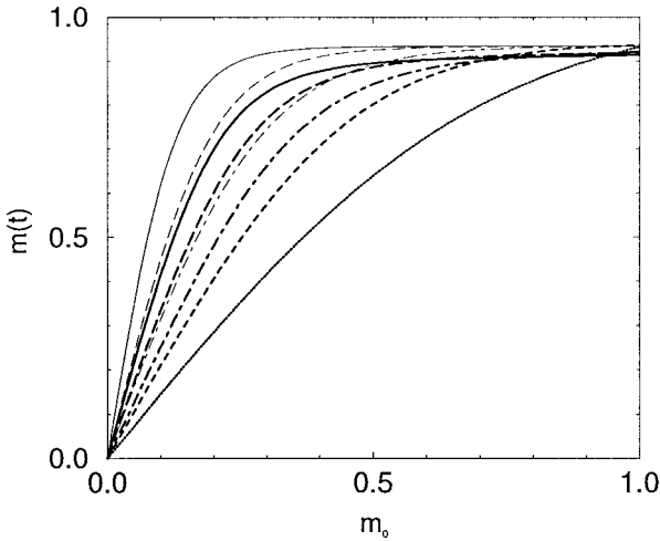
Fig. 1. The overlap m(t) for Q=2 systems is presented for the first five time steps as a function of m_0 for \alpha=0.3 . The results for the first, second, third, fourth and fifth time step are indicated by a dotted, a short-dashed, a dashed-dotted, a long-dashed and a full curve respectively. The results using the ansatz of ref. 7 for the third, fourth and fifth time step are indicated with thin lines.
