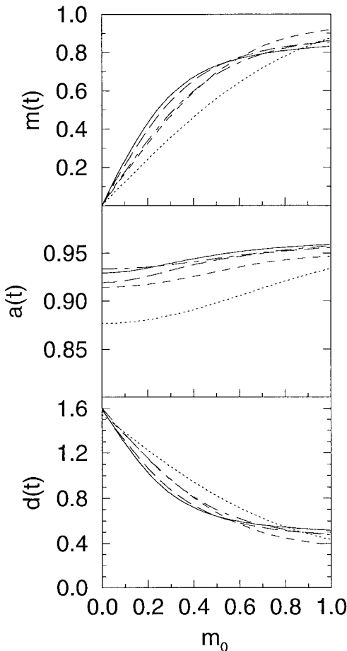
Fig. 3. The overlap m(t) , the activity a(t) and the Hamming distance d(t) are presented for the first five time steps as a function of m_0 for the network parameters b=0.1 , \alpha=0.5 , a_0=0.83 . The curves for the different time steps are as in Fig. 1
