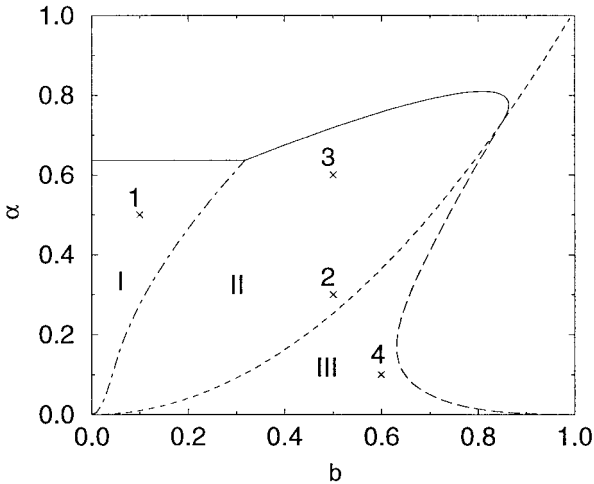
Fig. 2. The \alpha-b phase diagram for Q=3 . The full curve and long-dashed curve indicate the boundary of the retrieval region. The dashed-dotted curve denotes the boundary between the Ising-like region I and the other regions. The short-dashed curve represents the boundary between regions II and III. The points 1 to 4 indicate the network parameters used in the discussion of the dynamics.
