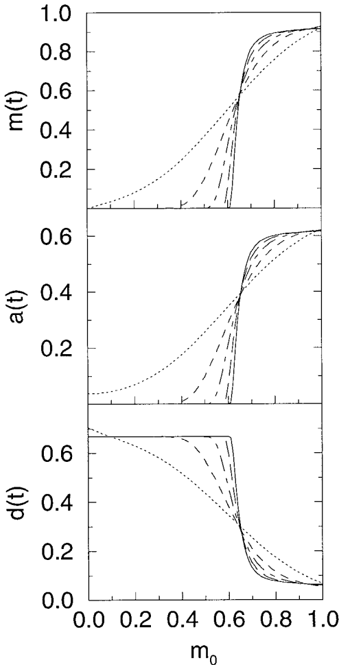
Fig. 5. As in Fig. 3, for the network parameters b = 0.6 , \alpha = 0.1 , a_0 = 0.83 .
