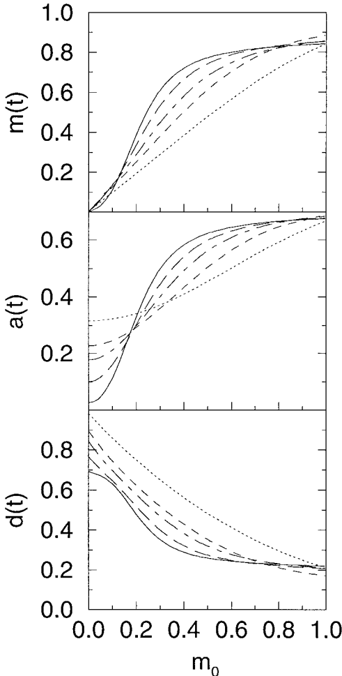
Fig. 4. As in Fig. 3, for the network parameters b = 0.5 , \alpha = 0.3 , a_0 = 0.83 .
